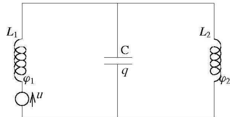
Figure 1: LC-circuit
