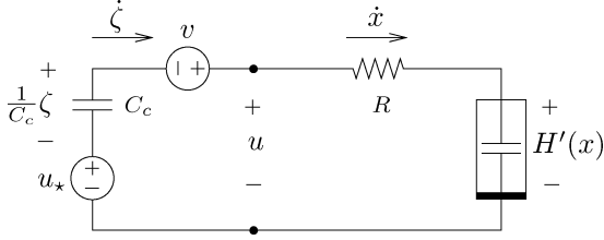
Fig. 6. Nonlinear RC circuit with controller.
