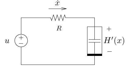
Fig. 4. Nonlinear RC circuit.
