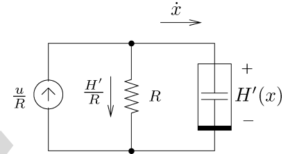
Fig. 5. Norton equivalent of the nonlinear RC circuit.
