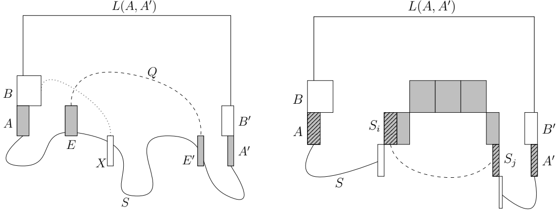
Figure 8: Proof of Lemma 9. Left: Step 1. The walk S satisfies (i) and connects A with A' . If from an inactive box X there is no inactive path to B (dotted line), then there is an active walk Q (dashed line) that connects active boxes E and E' in S on either side of X . Right: Step 2. The walk S satisfies (i) and contains no inactive boxes outside F . The boxes A , S_i , S_j and A' (striped) all belong to F' . The proof works by finding a path in F' from S_i to S_j (dashed line). In both figures active boxes are colored gray and inactive boxes are colored white.
