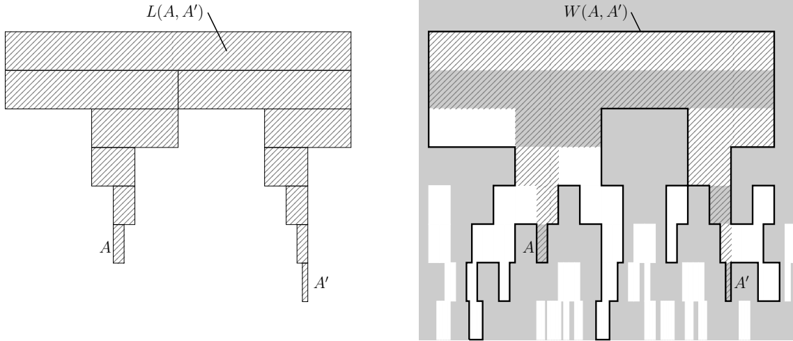
Figure 6: Two boxes A, A' in \mathcal{B} and the path L(A, A') that connects them (left). We can form L(A, A') by concatenating the shortest paths from A and A' to the lowest box lying above both A and A' . In the right image active boxes are colored gray and inactive boxes are colored white. The union of L(A, A') and the inactive components intersecting L(A, A') is called W(A, A') and outlined in black.
