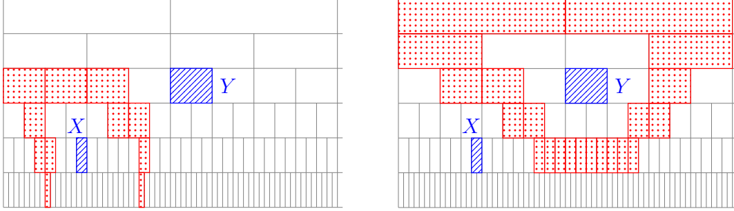
Figure 5: If two blue boxes X and Y are not connected by a path of blue (striped) boxes, then a red (dotted) walk exists that intersects every path in \mathcal{B} from X to Y (Lemma 6). This walk can be chosen such that it either connects two boxes in L_0 (left) or is cyclic (right).
