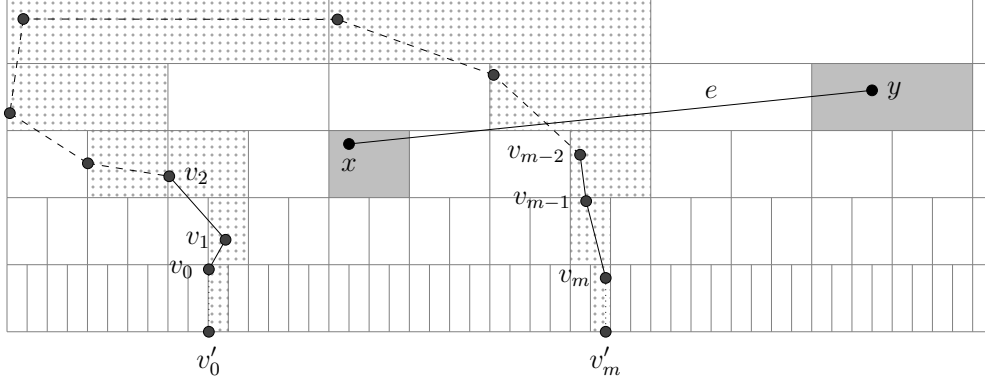
Figure 7: Proof of Lemma 8. The edge e of \Gamma connects vertices x and y . If a red (dotted) walk of boxes exists that separates the boxes containing x and y , then e intersects one of the segments [v_i, v_{i+1}] , [v_0, v'_0] or [v_m, v'_m] . This contradicts the assumption that no red box contains a neighbor of x or y .
