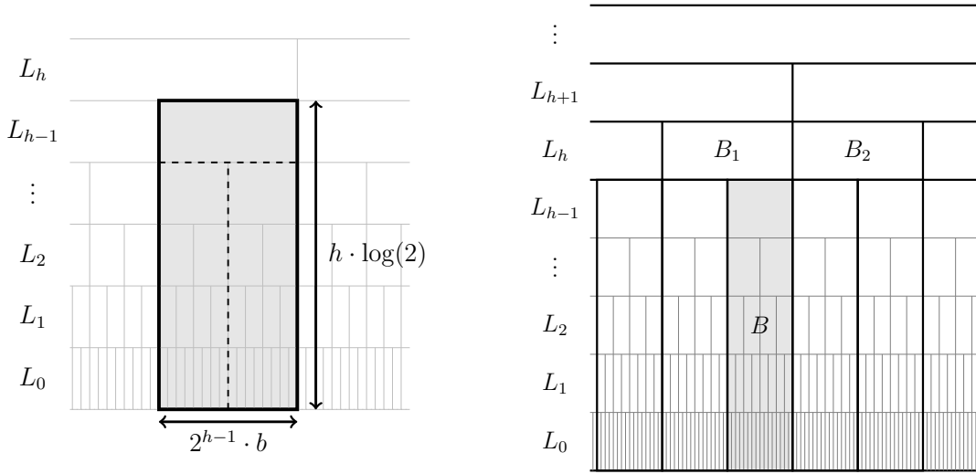
Figure 9: Left: an h -block (in the figure h = 5 ). An h -block is the union of 2^h - 1 boxes in the lowest h layers. Right: definition of a lonely block (used in the proof of Lemma 16). The lowest h layers are partitioned into h -blocks. An h -block B in W' is called lonely if both boxes B_1 and B_2 lying above it are not in W' . If |W'| > 3 and B is lonely, one of the blocks adjacent to B contains a horizontal path in W .
