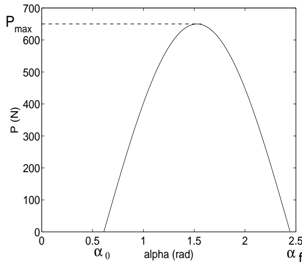
Figure 6.1: Force on the Oarhandle During the Power Stroke
