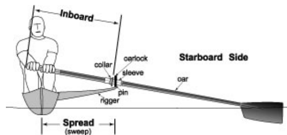
Figure B.2: Sweep Diagram
