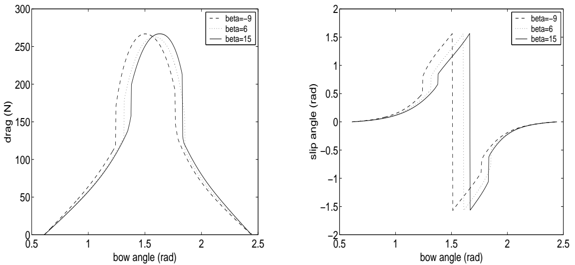
Figure 8.8: Three Blade Cant Angles: Drag Force and Slip Angle
