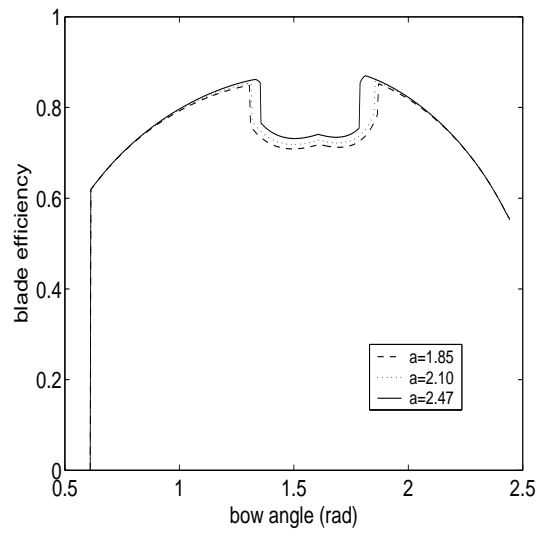
Figure 8.6: Three Oarlengths: Blade Efficiency
