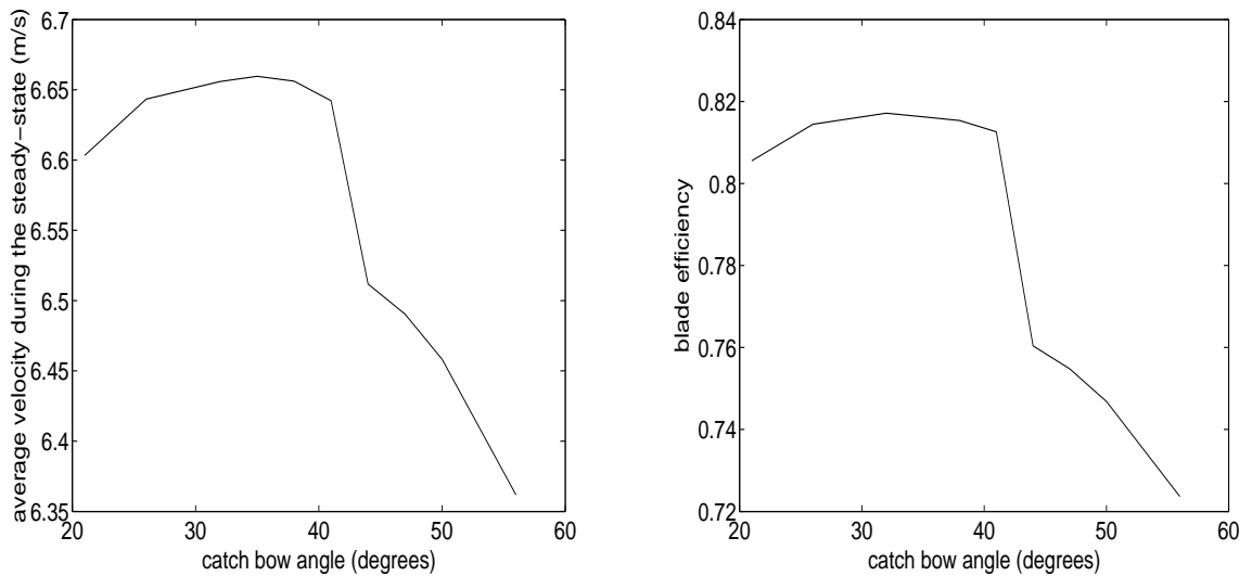
Figure 8.10: Effect Catch Bow Angle on Boat Velocity and Blade Efficiency
