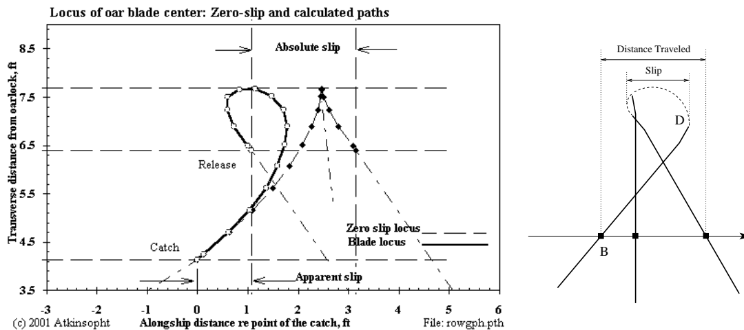
Figure 1.2: Left: Zero-Slip Path and Slip Path (8+ Heavy Men, from Akinson [9]), Right: Oar and Blade with Slip Path
