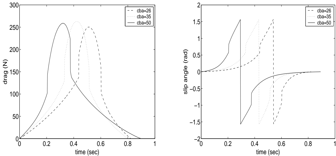
Figure 8.11: Three Catch Bow Angles: Drag Force and Slip Angle
