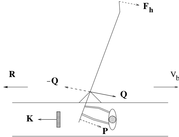
Figure 3.2: Forces on Boat and Rower
