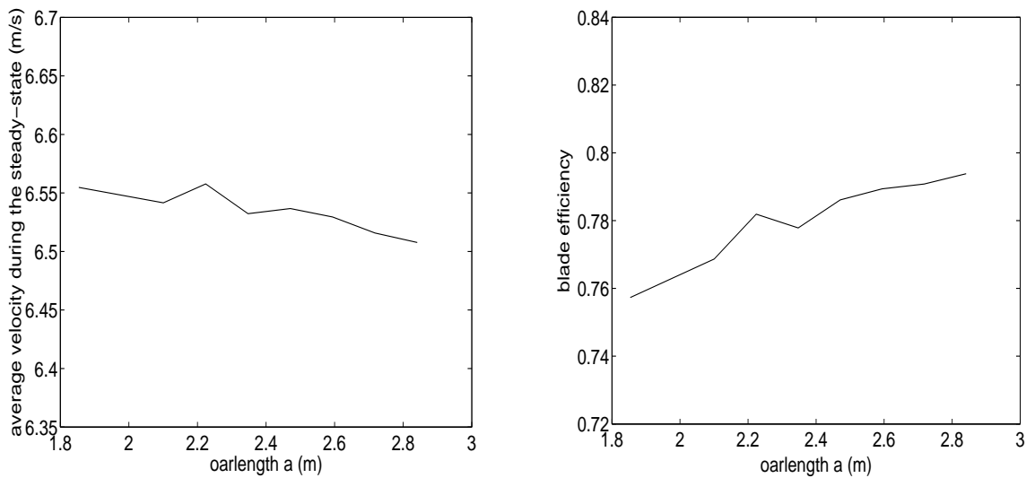
Figure 8.4: Effect Oarlength on Boat Velocity and Blade Efficiency
