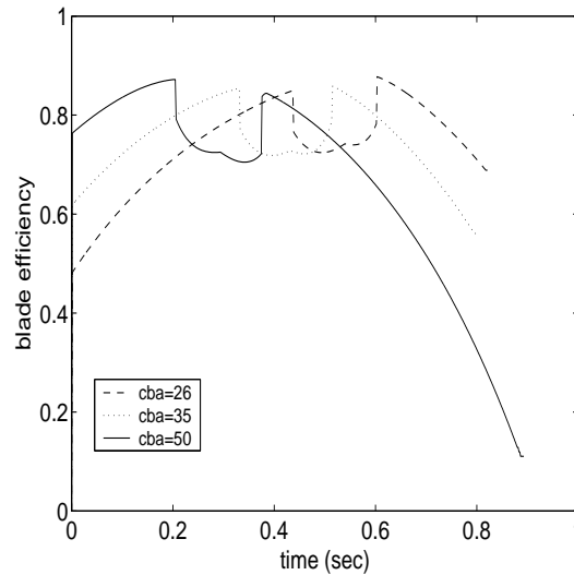
Figure 8.12: Three Catch Bow Angles: Blade Efficiency
