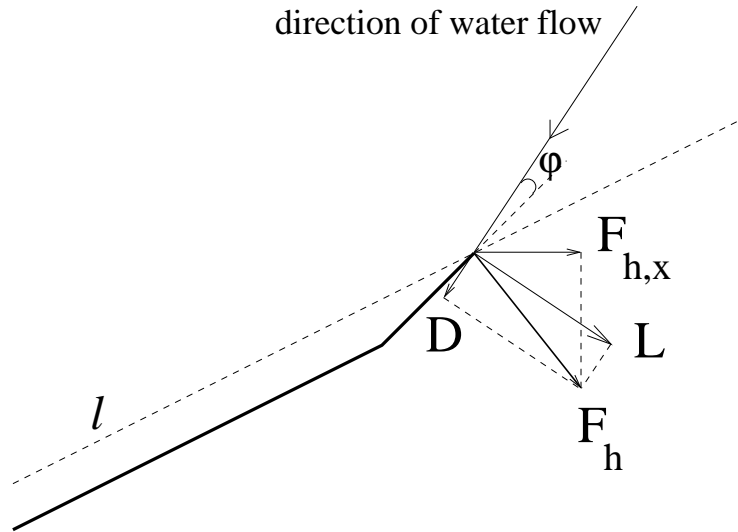
Figure 2.4: Blade Forces
