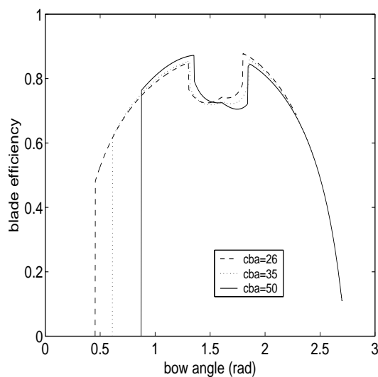
Figure 8.14: Three Catch Bow Angles: Blade Efficiency
