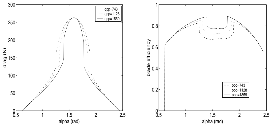
Figure 8.2: Three Blade Sizes: Drag Force and Blade Efficiency
