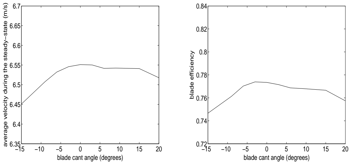
Figure 8.7: Effect Blade Cant Angle on Boat Velocity and Blade Efficiency
