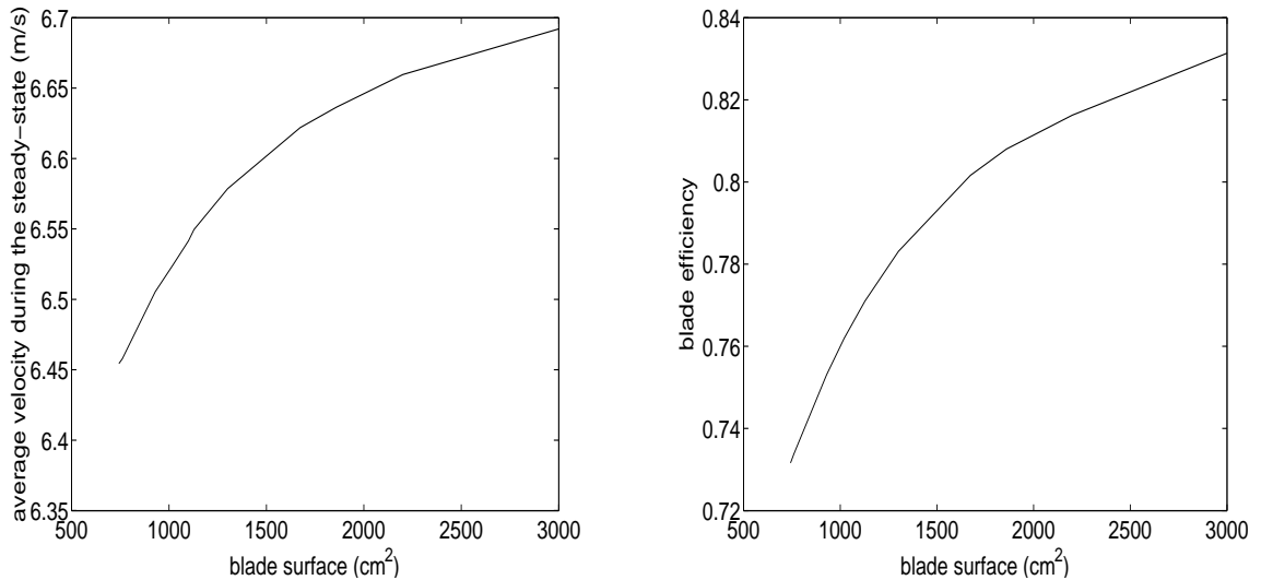
Figure 8.1: Effect Oar Blade Surface on Boat Velocity and Blade Efficiency
