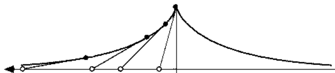
Figure 1.3: Tractrix
