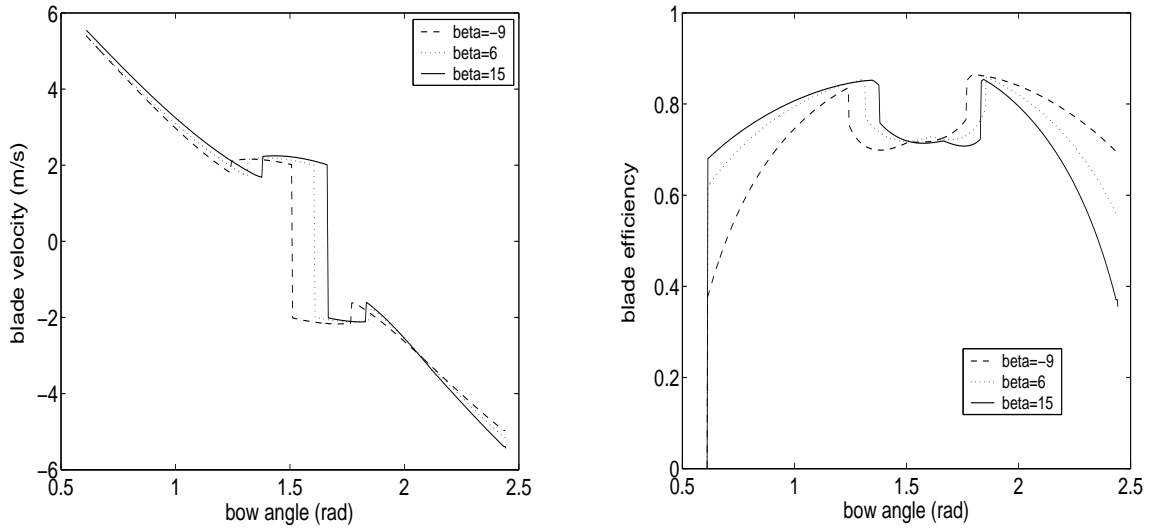
Figure 8.9: Three Blade Cant Angles: Blade Velocity and Blade Efficiency
