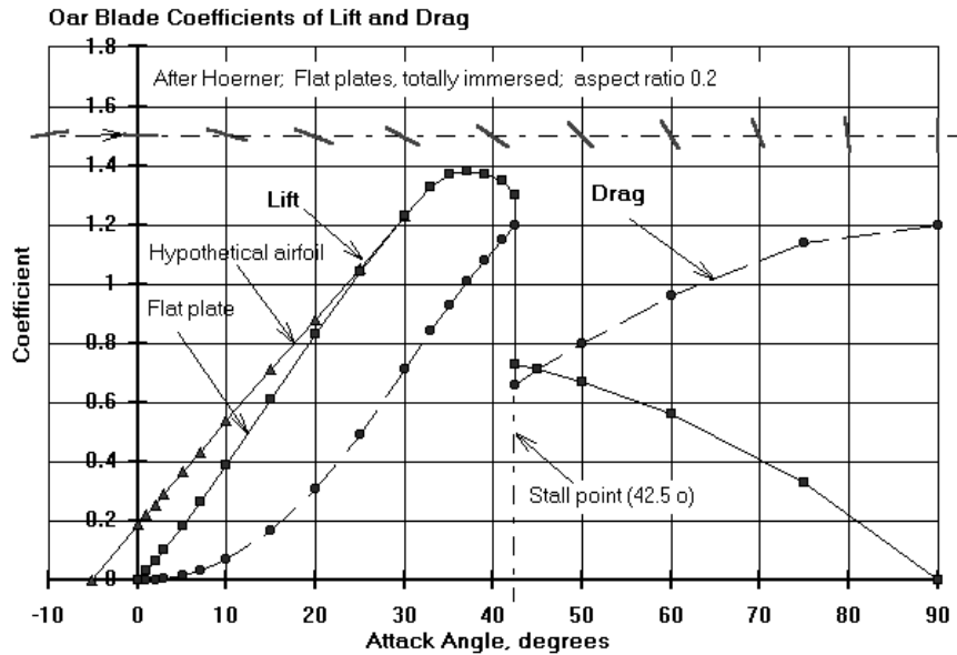
Figure 2.5: Oar Blade Coefficients of Lift and Drag (from [9])
