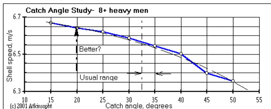
Figure 8.16: Catch Angle Study 8+ heavy men (from Atkinson [9])
