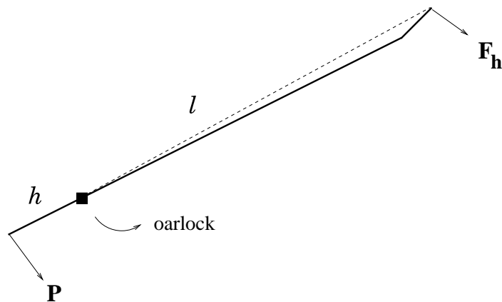
Figure 2.2: Moments about the Oarlock
