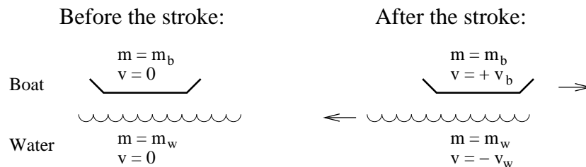
Figure 3.1: Change in Momentum
