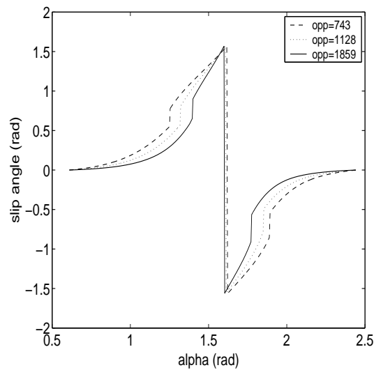
Figure 8.3: Three Blade Sizes: Slip Angle
