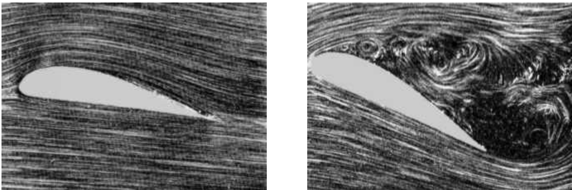
Figure 2.6: Left: Attached flow around an airfoil at small angles of attack, Right: Separated flow around an airfoil at high angles of attack (stall)
