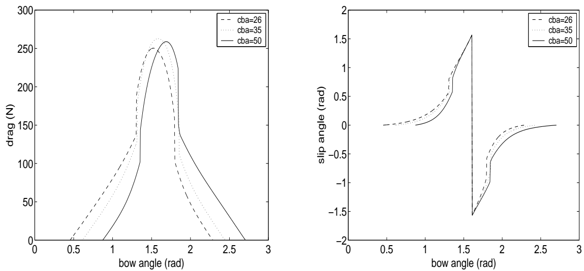
Figure 8.13: Three Catch Bow Angles: Drag Force and Slip Angle
