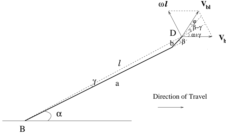
Figure 1.4: Oar and Blade Displacements
