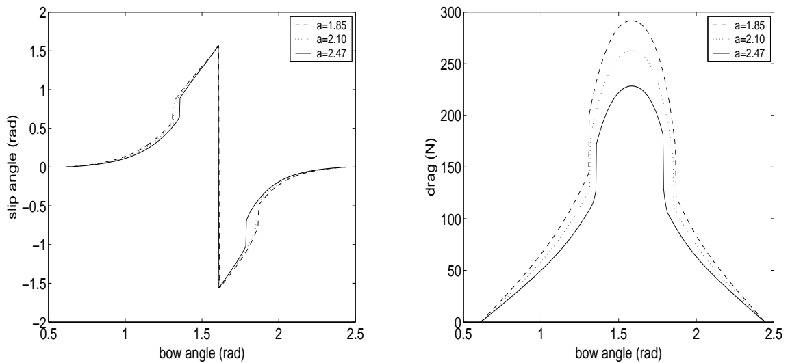
Figure 8.5: Three Oarlengths: Slip Angle and Drag Force
