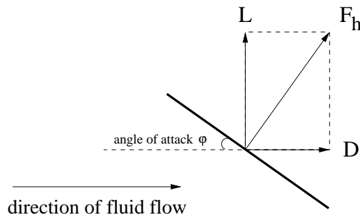
Figure 2.3: Forces on a Flat Plate
