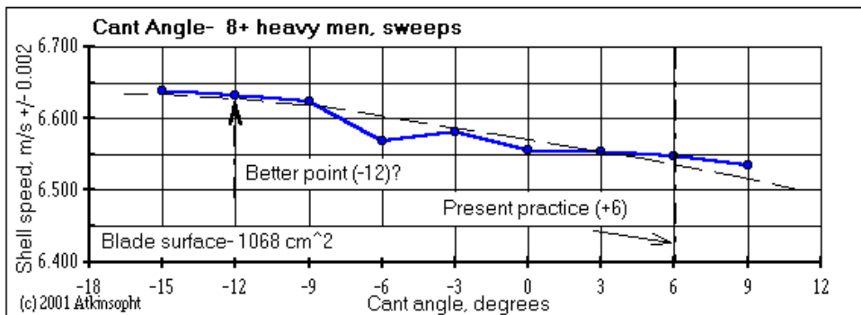
Figure 8.15: Cant Angle Study 8+ heavy men (from Atkinson [9])
