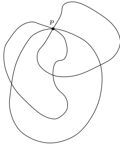
Figure 30: A pencil pseudocircle arrangement.
