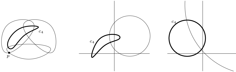
Figure 17: The arrangement (c_1, c_2, c_3) is as in Figure 6, right, and c_4 intersects two sides of a 2-face.
